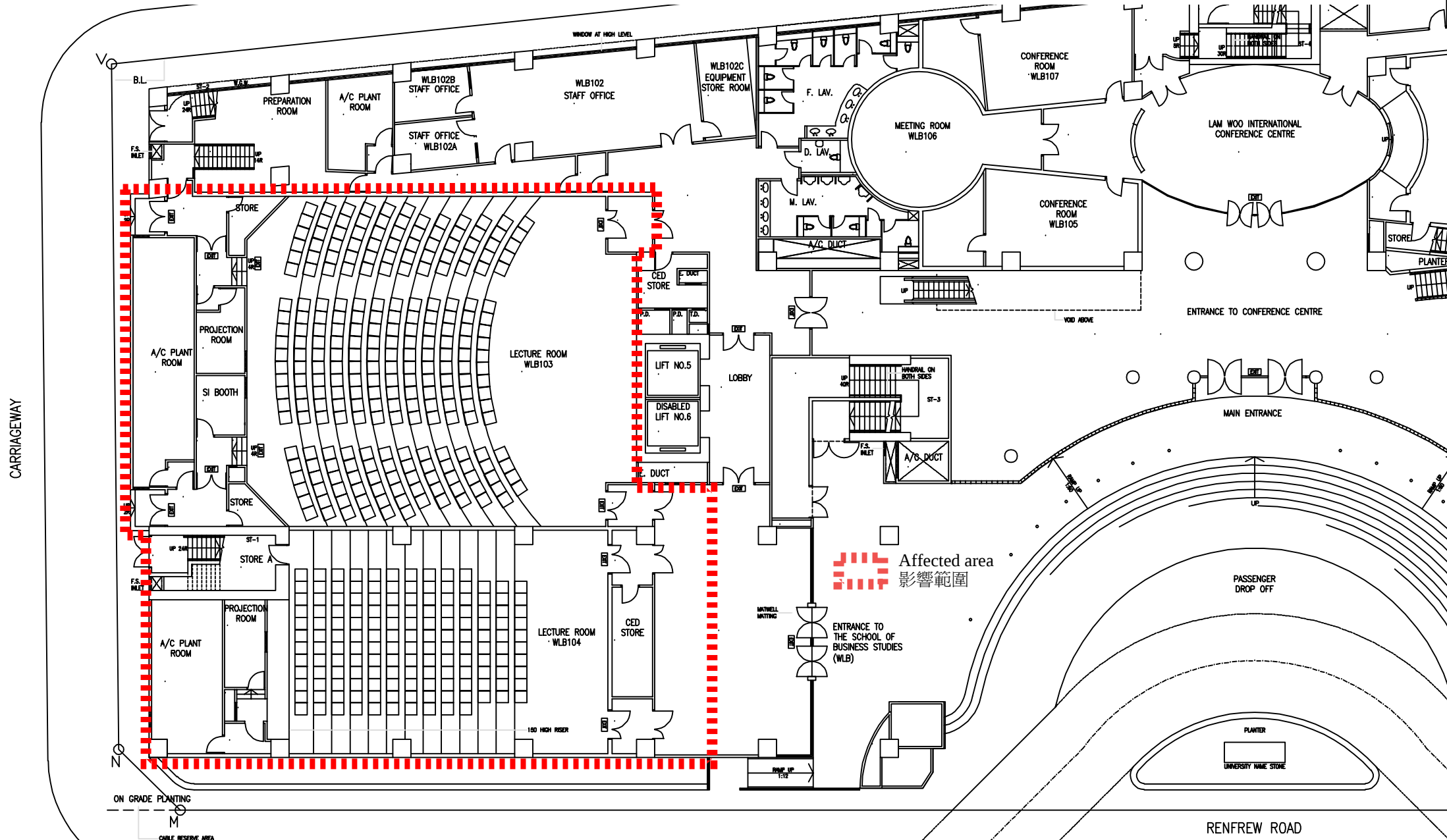
Layout Plan of Level 1 of The Wing Lung Bank Building for Business Studies (WLB)
