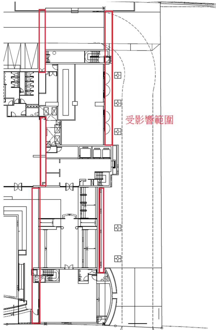
Layout plan of LG/F, SRH North Building
