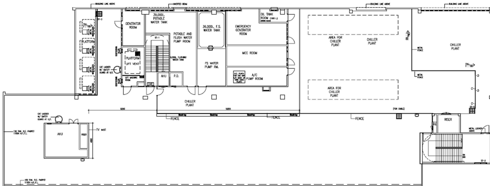
Layout plan of Roof, Communication and Visual Arts Building
