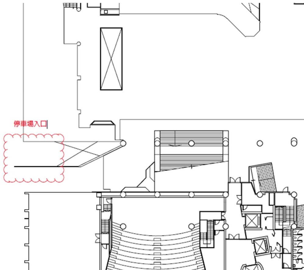
Layout plan of Level 5 of Fong Shu Chuen Car Park entrance
